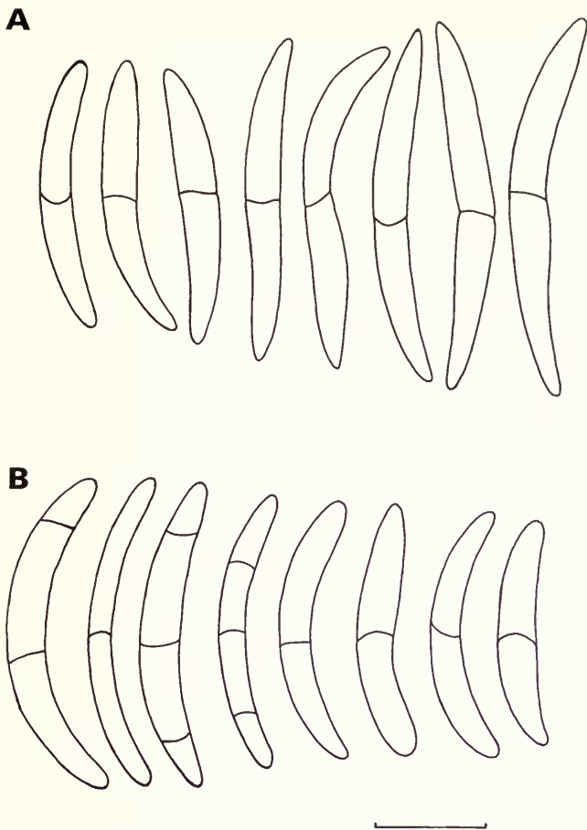
Fig. 2 Ascospore outlines (A) Leptorhaphis amygdali (Massal.) Zwackh (PAD-isolectotype); (B) Leptorhaphis atomaria (Ach.) Szat. (H-ACH 795a-lectotype); scale = 10 µm.
